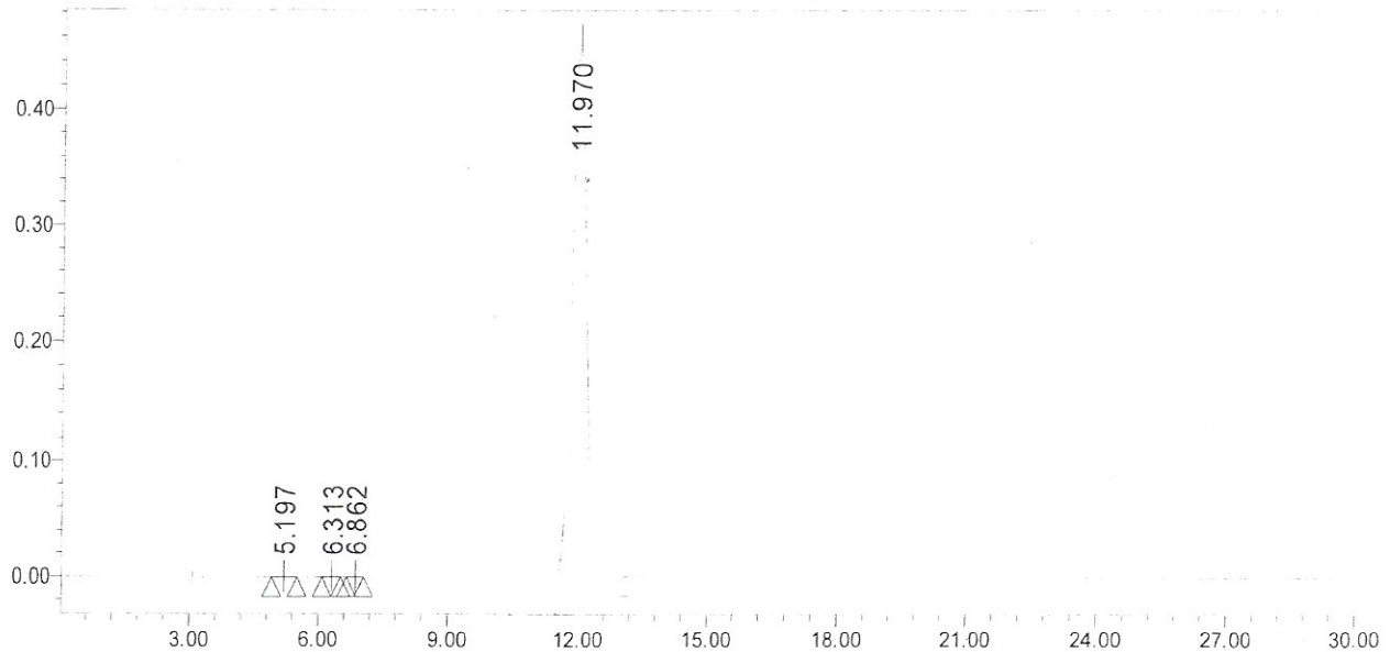
Auto-Scaled Chromatogram
